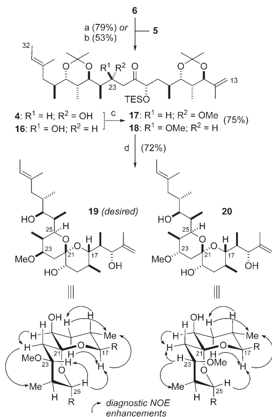
Scheme 4. Aldol coupling and spiroacetalization. a) LDA, THF, -78^{\circ}\text{C} , 1 h; 5, -78^{\circ}\text{C} , 1 h; b) 1. (-)\text{-Ipc}_2\text{BCl} , \text{Et}_3\text{N} , \text{Et}_2\text{O} , 0^{\circ}\text{C} , 1 h; 5, -78^{\circ}\text{C} , 2 h; 2. MeOH, pH 7 buffer, \text{H}_2\text{O}_2 ; c) \text{Me}_3\text{OBF}_4 , proton sponge, \text{CH}_2\text{Cl}_2 , 0\rightarrow 20^{\circ}\text{C} , 2 h; d) CSA, MeOH, 20^{\circ}\text{C} , 16 h. CSA = camphorsulfonic acid; Ipc = isopinocampheyl.
